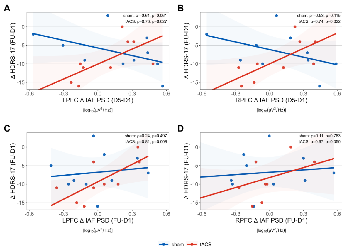
Figure 2. Target Validation: Early and Sustained Prefrontal Alpha Modulation Predicts Depressive Symptom Improvement at 2-Week Follow-Up. A–D: Spearman correlations between changes in prefrontal alpha power at the individual alpha frequency (IAF PSD) and depressive symptom change (HDRS-17), shown separately for sham and tACS groups. Panels A (LPFC) and B (RPFC): IAF PSD change during the intervention week (D5–D1) in relation to HDRS-17 change (FU–D1). Panels C (LPFC) and D (RPFC): IAF PSD change from Day 1 to follow-up (FU–D1) in relation to HDRS-17 change (FU–D1). Lines represent linear regression fits with shaded 95% confidence intervals.
