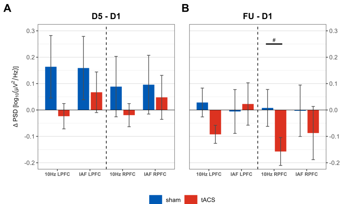
Figure 1. Target Engagement: ROI Analysis of Alpha PSD Modulation. Difference scores for left (LPFC) and right (RPFC) prefrontal electrode seeds have been calculated for IAF and 10 Hz PSD respectively. A: Alpha PSD change within the intervention week (D5-D1); B: Alpha PSD Change from Day 1 to 2-week follow-up (FU-D1). Error bars represent standard error of the mean. #: p = 0.066 .
